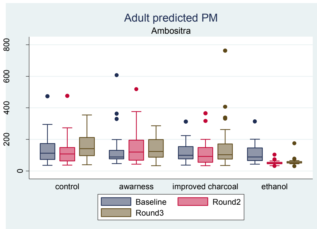
Figure 10-3: Distributions of adult predicted PM 2.5 (µg/m 3 ) at Baseline, Round 2 and Round 3 by intervention group - Ambositra
